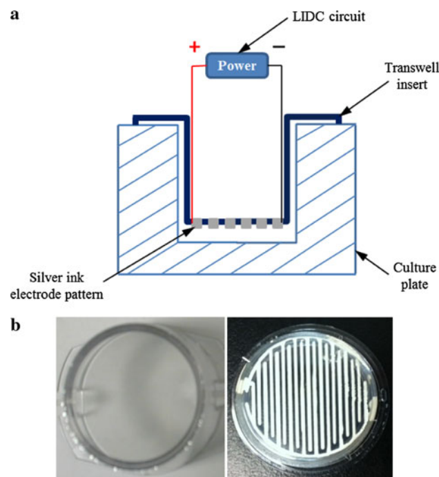
Fig. 1 a Schematic of electrode testing configuration in a cell culture plate. b Blank Transwell insert (left) and silver ink printed onto the bottom of Transwell insert (right)
