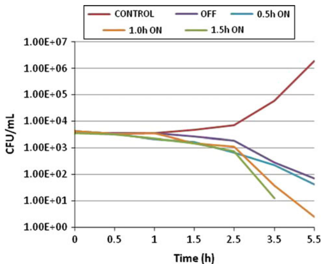
Fig. 5 Bacterial killing curves for Staphylococcus aureus exposed to silver electrodes, with or without 28 \mu\text{A} current, for up to 1.5 h
