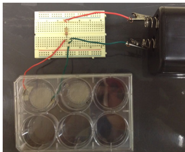
Fig. 2 Overview of apparatus, showing six-well plate, battery and waffle board, all mounted on an acrylic plate. Silver electrodes printed onto the bottom of Transwells in upper left well (with 28 μA current applied) and in upper middle well (no current applied), with an open well control in upper right
