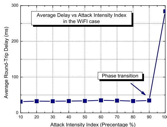
Fig. 7. The mean round-trip delay of DNP3 packets for different values of the attack intensity indexes in the WiFi case.
