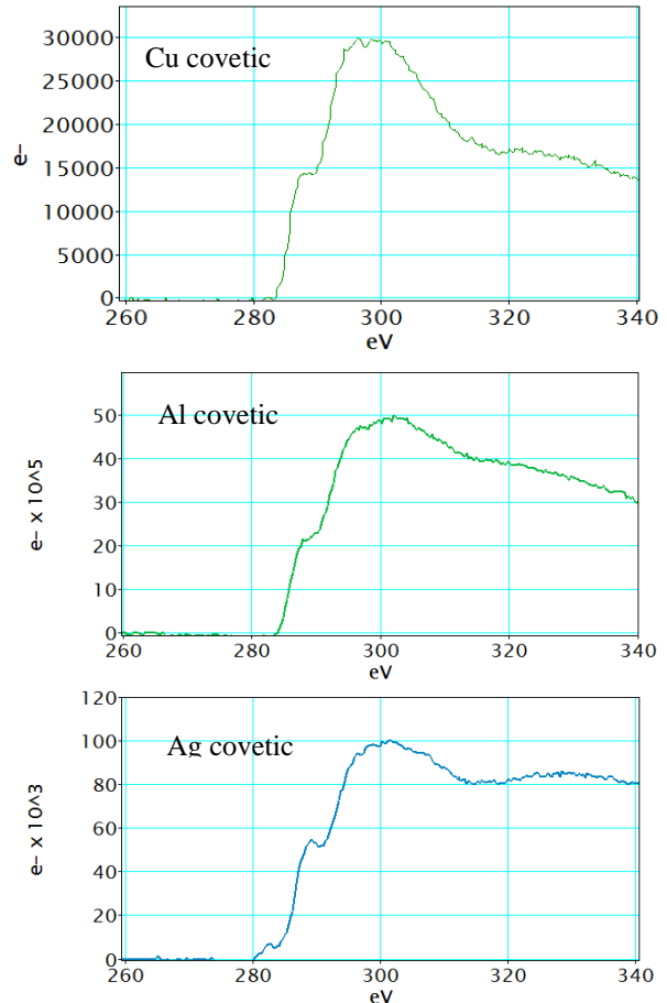
Fig. 6 EELS spectra at the C-K edge from Cu, Al and Ag covectics.
