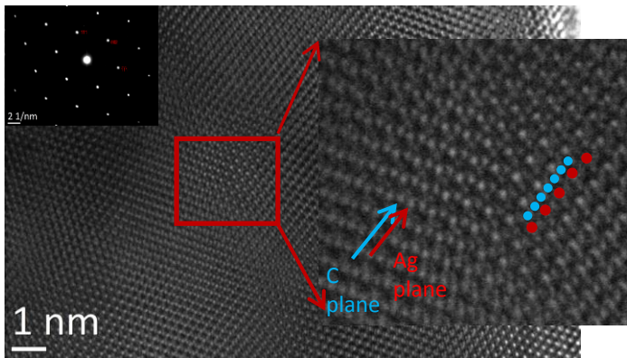
Fig. 5 [1 \bar{1} 0] HRTEM image of Ag cv 3%. A region showing alternating planes between the Ag (111) planes is enlarged. This region seems to have graphene planes embedded in the Ag lattice. The inset is the diffraction pattern from the area.
