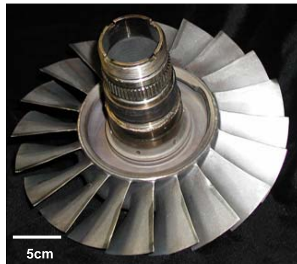
Figure 14. Blisk repair, post finishing, for T700 Engine.
