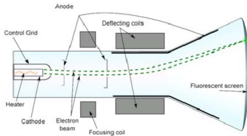
Figure 5. Cathode Ray Tube (CRT) [From ShareAlike 3.0]
