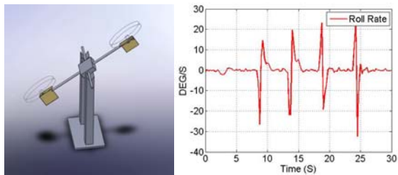
Fig. 6. Propulsion test stand and response to impulse
