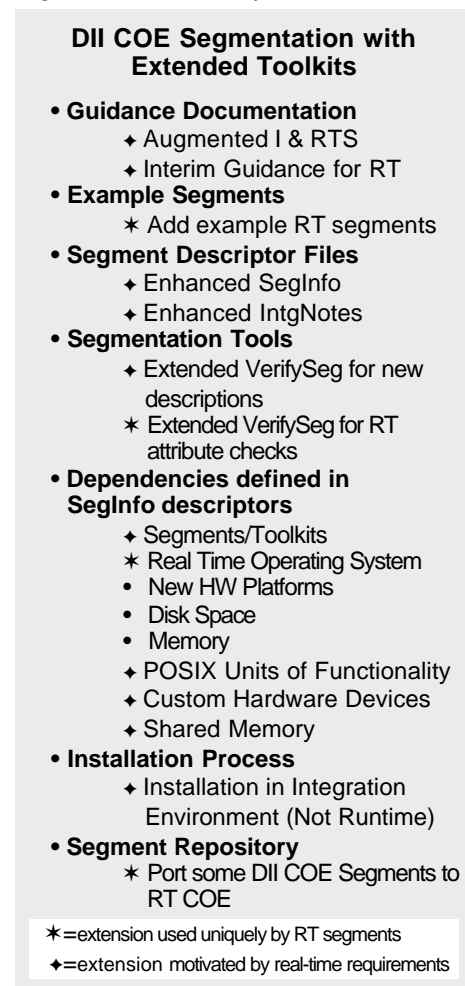
Figure 5: Process and Information Extensions
