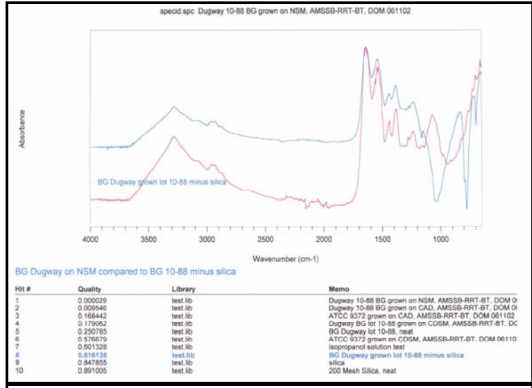
Figure 4: TravelIR Infrared spectral analysis of BG grown on NSM medium (bottom) as compared to the spectra from Dugway stocks (top) after subtraction of
