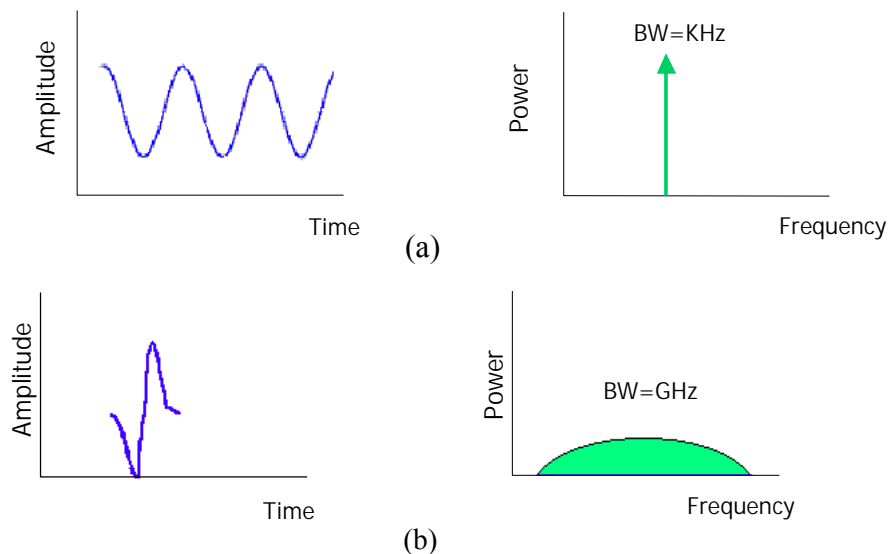
Figure 4. (a) Conventional narrowband communications send long continuous waveforms and generate very narrow frequencies. (b) UWB communications send extremely narrow pulses and generate very wide frequencies.
