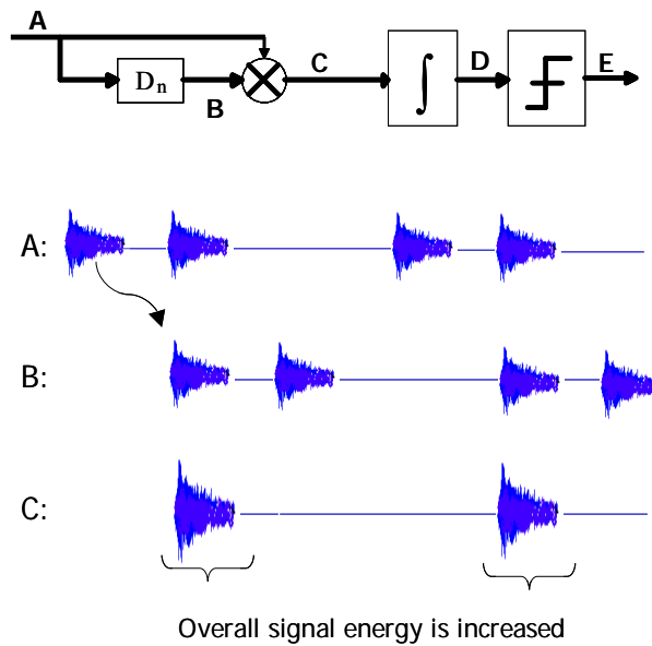
Figure 7. TR receiver diagram and its signal representation in a multipath propagation channel
