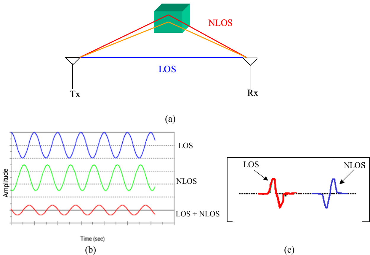
Figure 5. (a) Multipath phenomenon in wireless channels (b) Multipath effect on narrowband signals (c) multipath effect on ultra-wideband pulses
