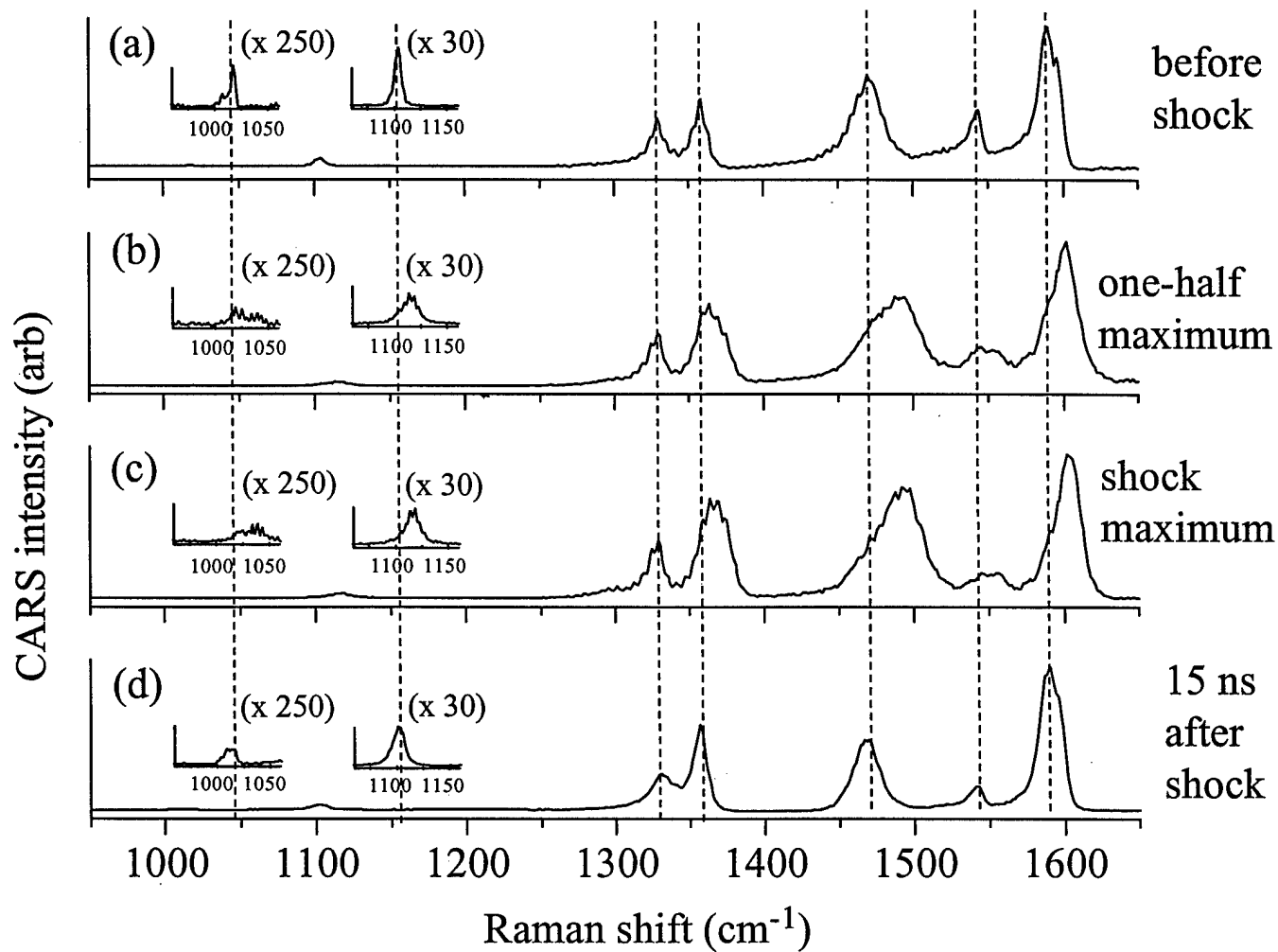
Figure 1. Ultrafast CARS spectrum of a polycrystalline film of NTO with a 4 GPa shock. After the 1 ns shock, the intensities of some transitions change on the ~5 ns time scale, indicating shock induced orientation of the nanocrystals.
