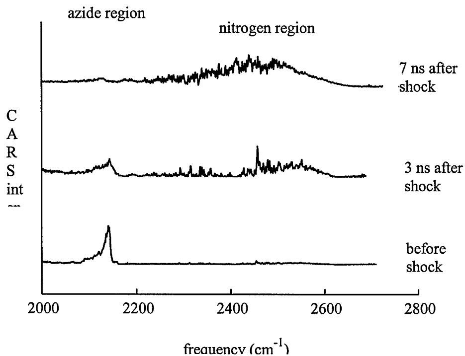
Figure 2. Ultrafast CARS spectrum of a \sim 4 GPa shock going through a thin film of C_3N_{12} . Before shock only the azide symmetric stretch is seen at \sim 2160 cm^{-1} . The broad region which appears is attributed to condensed phase N_2 in a badly damaged crystal lattice.
