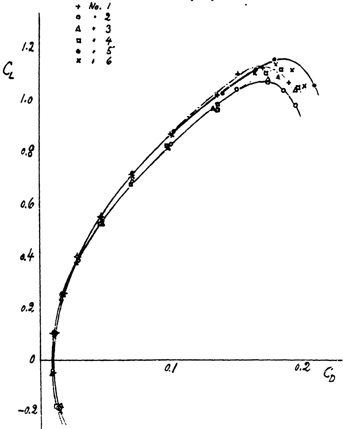
Fig. 6.- Wind Tunnel Measurements on a Rectangular 2412 Wing, Equipped with 6 Different Tip Caps as Shown in Fig. 2. Aspect Ratio A = 3.0 ; R = 2.10^6 ; Ref. 3.
