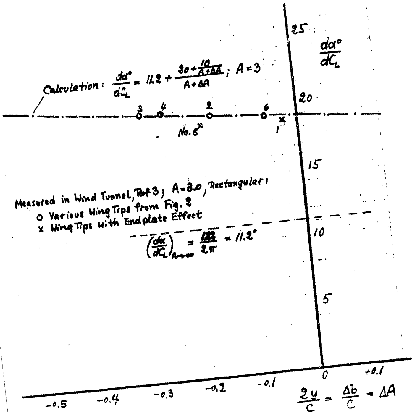
Fig. 3.- The Variation of the Lift Curve Slope with the Effective Aspect Ratio A; = A + \Delta A ; According to Theory, and from Experiments.
