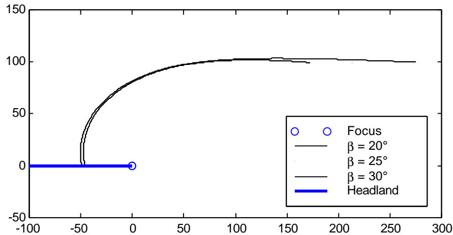
Fig. 7. Sensitivity of parabolic shape to selection of control point location.
