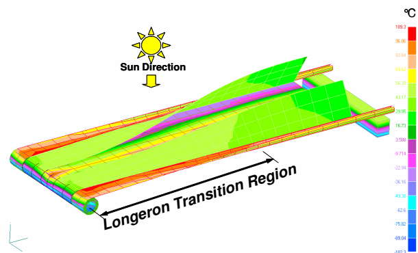
Figure 10 - Steady-state RAPDAR™ thermal analysis.
