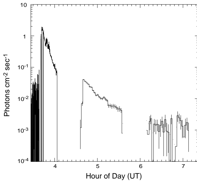
Figure 1. Time profile of the 2.223 MeV neutron-capture line.
