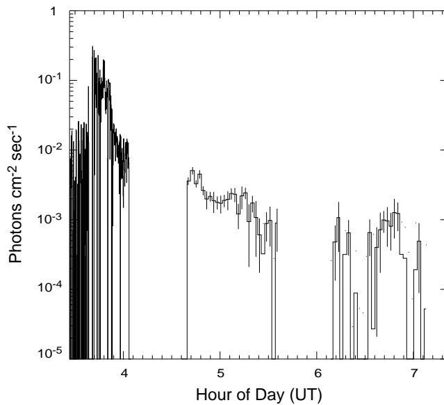
Figure 2. Time profile of the 4.44 MeV ^{12}\text{C} nuclear deexcitation line.
