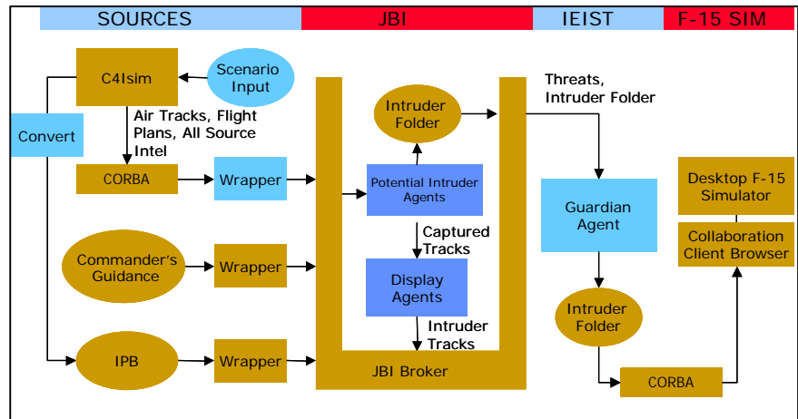
Figure 7. IEIST/Y-JBI Prototype
