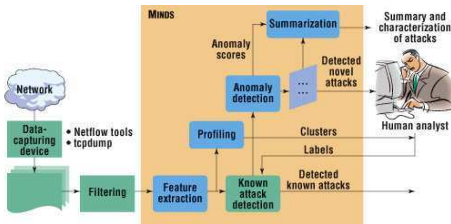
Fig. 1. The Minnesota Intrusion Detection System (MINDS)
