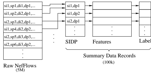
Fig. 3. Transformation of raw netflow data in an observation window to the Summary Data Set. Features are constructed using the set of netflows in the observation window. Labels for use in the training and test sets are constructed by analyzing the data over a long period (usually several days)
