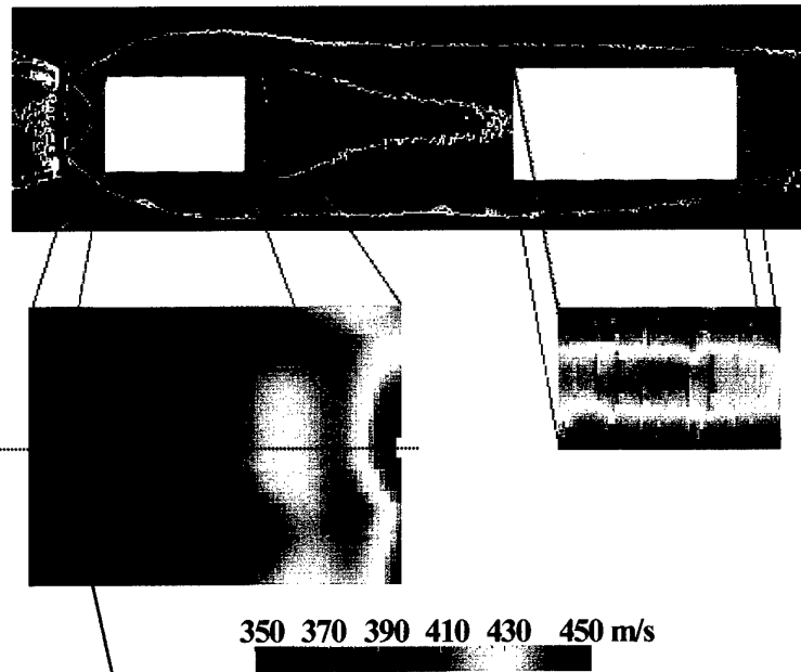
Fig. 13 Velocity distributions in pseudo colors
