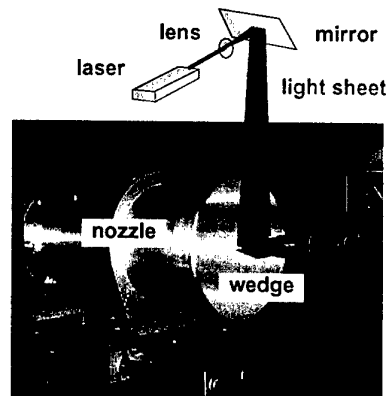
Fig. 18 Shock tunnel nozzle, wedge arrangement and illumination
