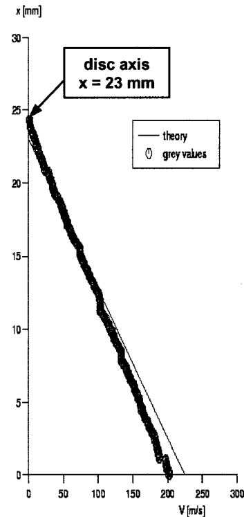
Fig. 8 Velocity distribution
