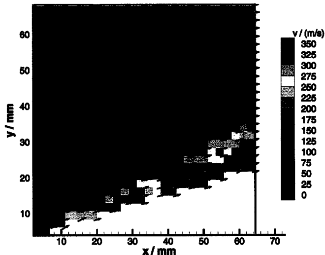
Fig. 24 Vertical velocity distribution measured with PIV
