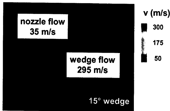
Fig. 25 Calibrated DPV velocity picture in terms of pseudo colours
