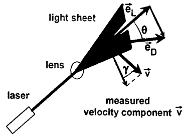
Fig. 1 Doppler effect
