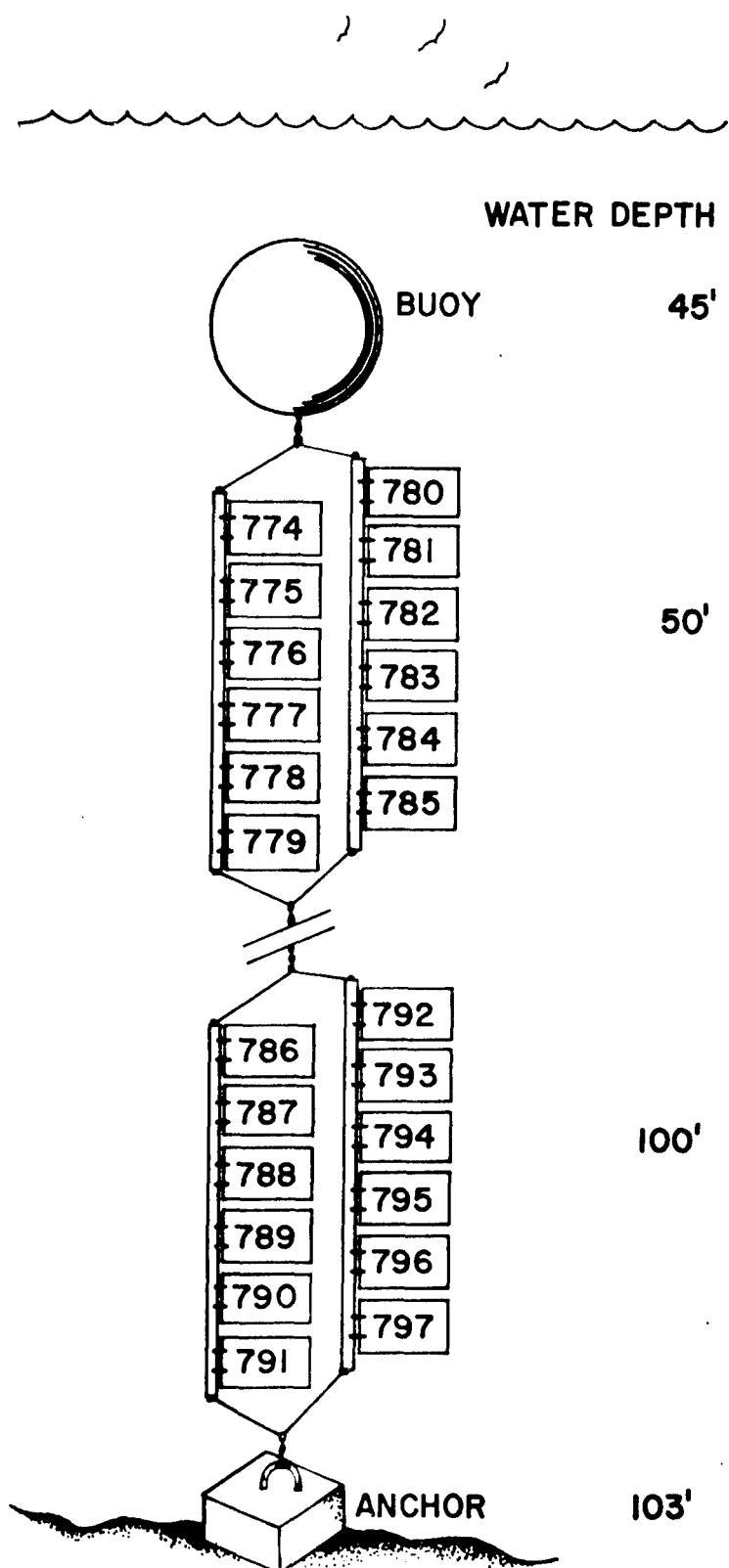
FIGURE 2. Configuration of Test Panel Array.
